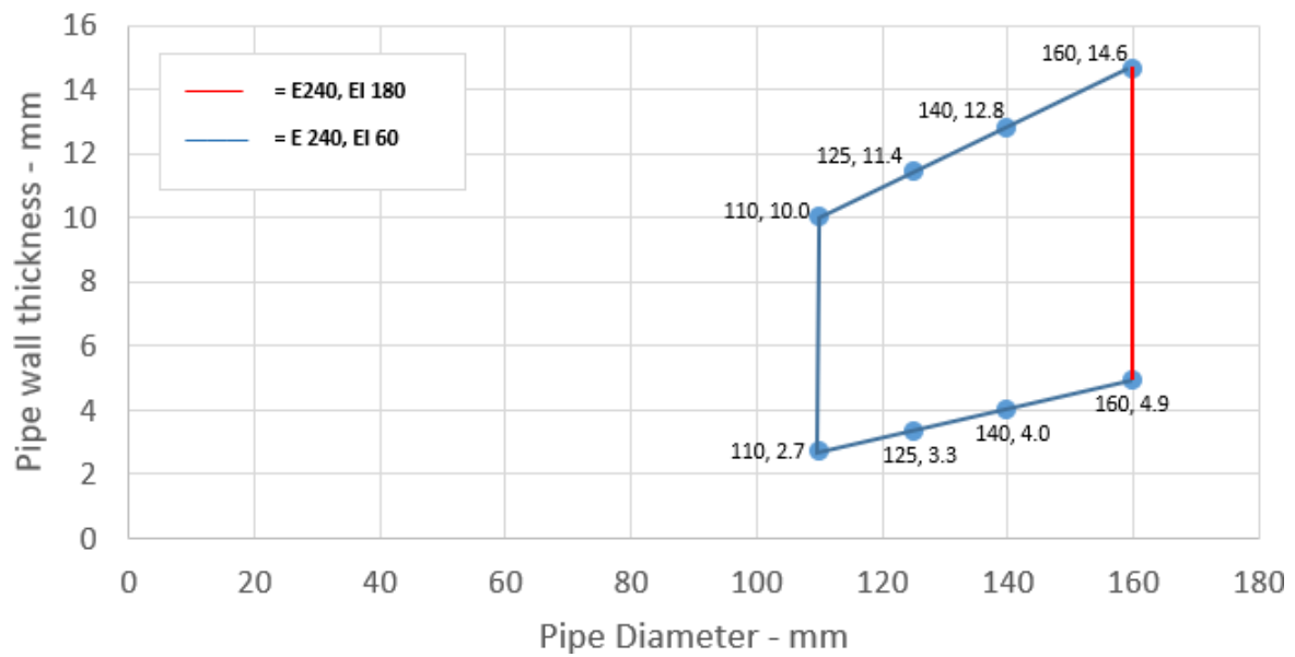
Figure 43 Intermediate pipe wall thicknesses for PP pipe diameters
