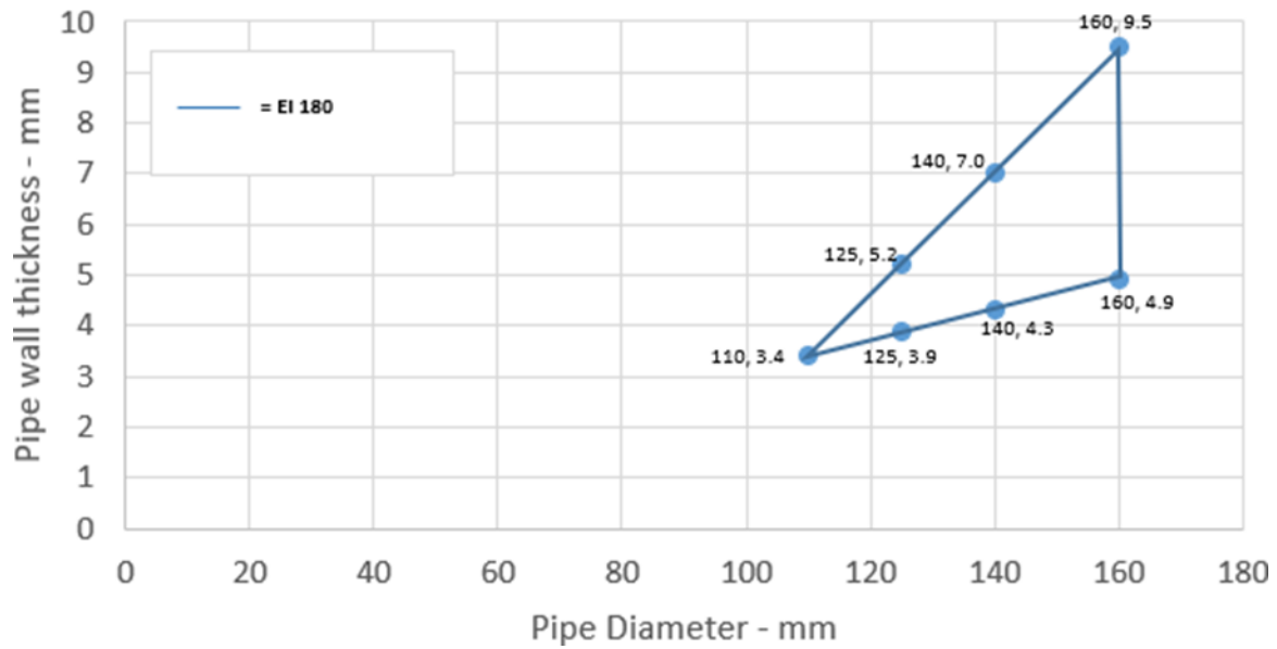
Figure 35 Intermediate pipe wall thicknesses for PE pipe diameters
