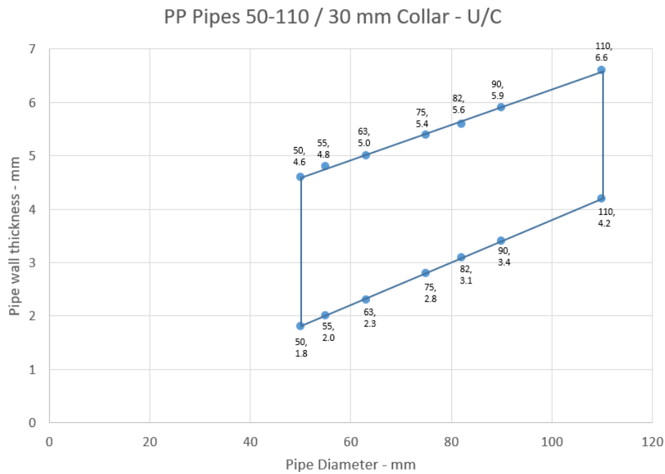
Figure 61 Intermediate pipe wall thicknesses for PP pipe diameters
