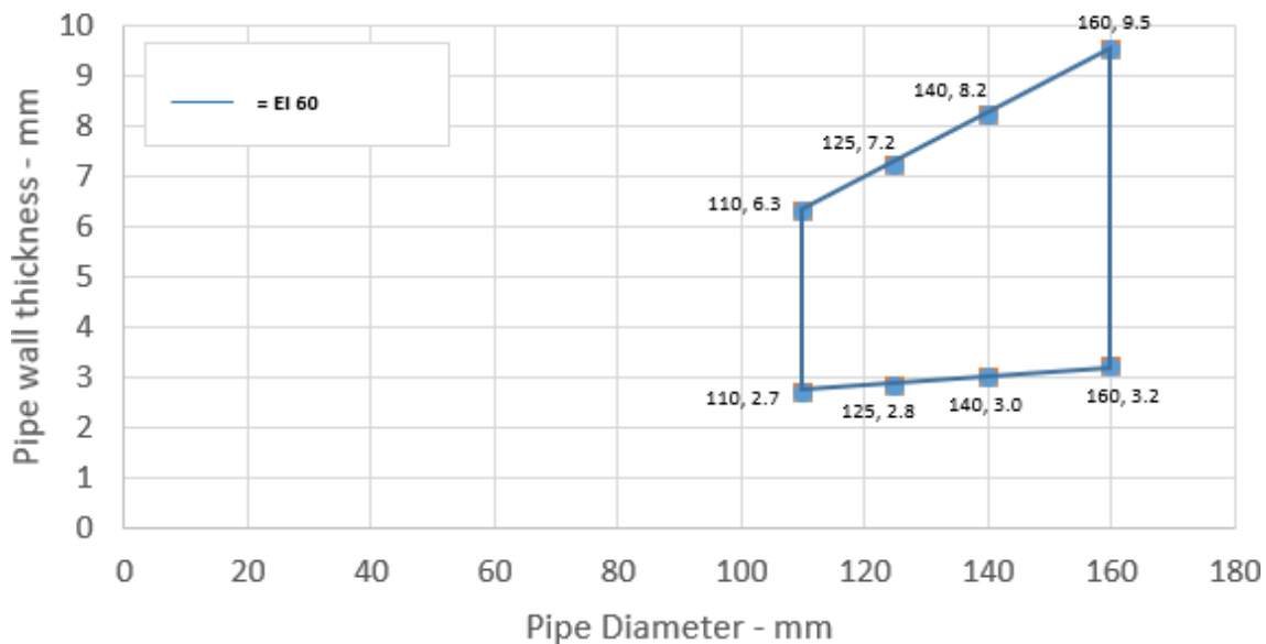
Figure 52 Intermediate pipe wall thicknesses for PVC pipe diameters
