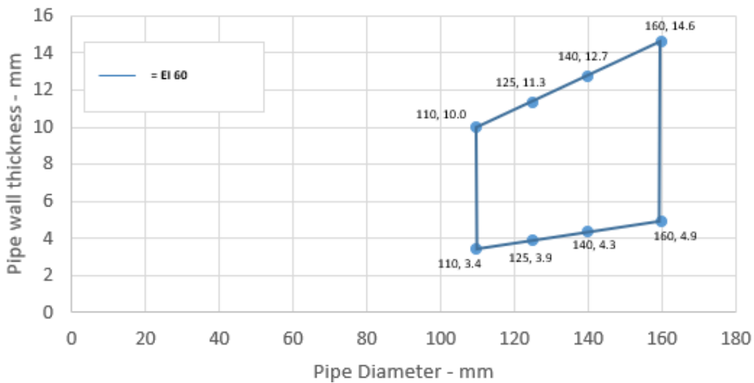
Figure 58 Intermediate pipe wall thicknesses for PE pipe diameters
